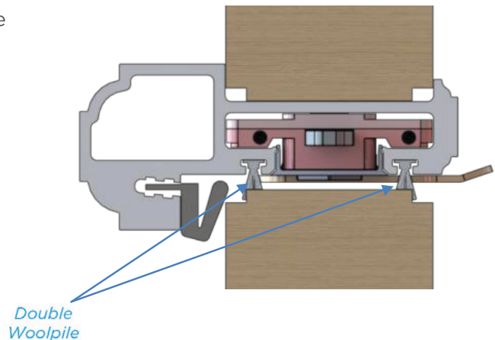
TOP VIEW, AS INSTALLED
