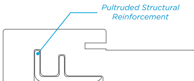
JAMB WITH REINFORCEMENT
