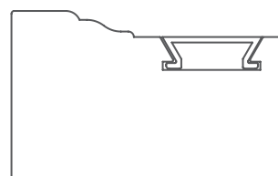
BRICKMOLD WITH NAIL COVER
