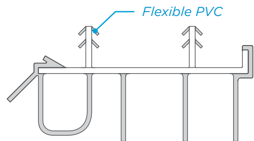
DRIVE-IN SWEEP
