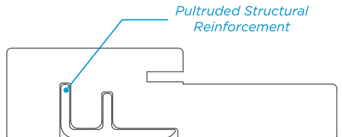
JAMB WITH REINFORCEMENT
